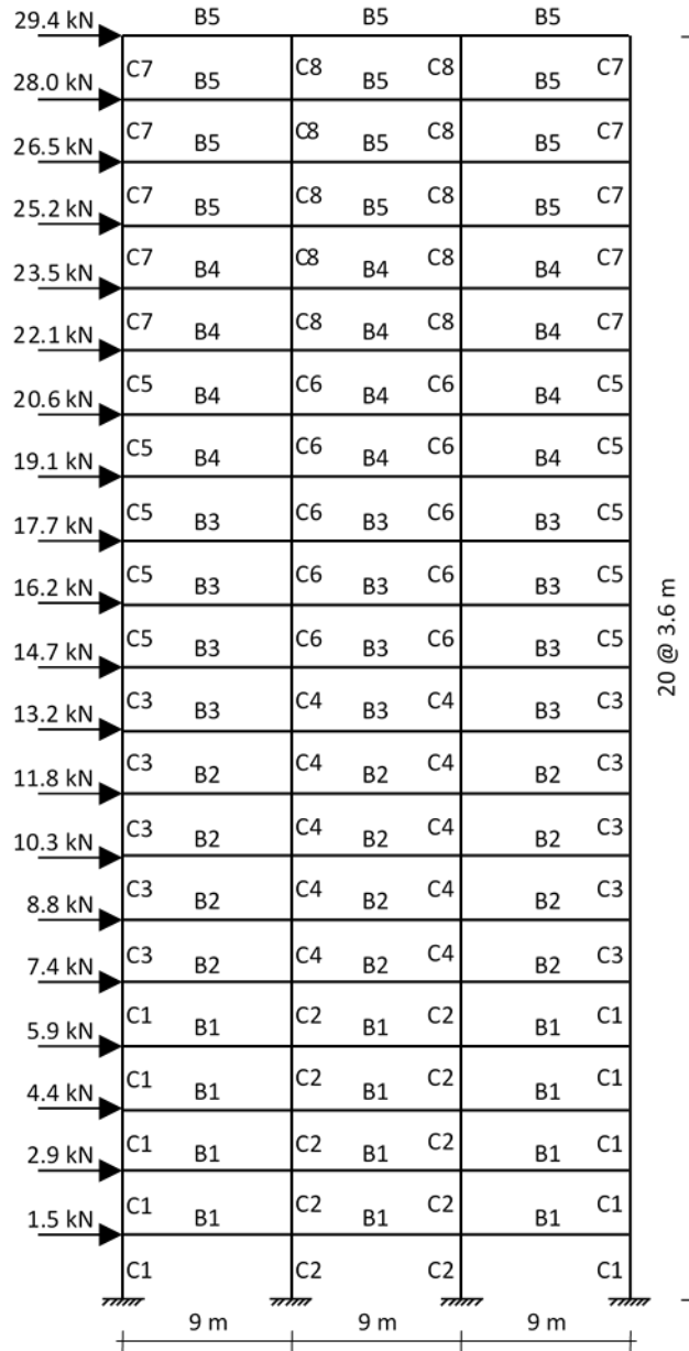
Figure 10. Twenty-story RC frame
