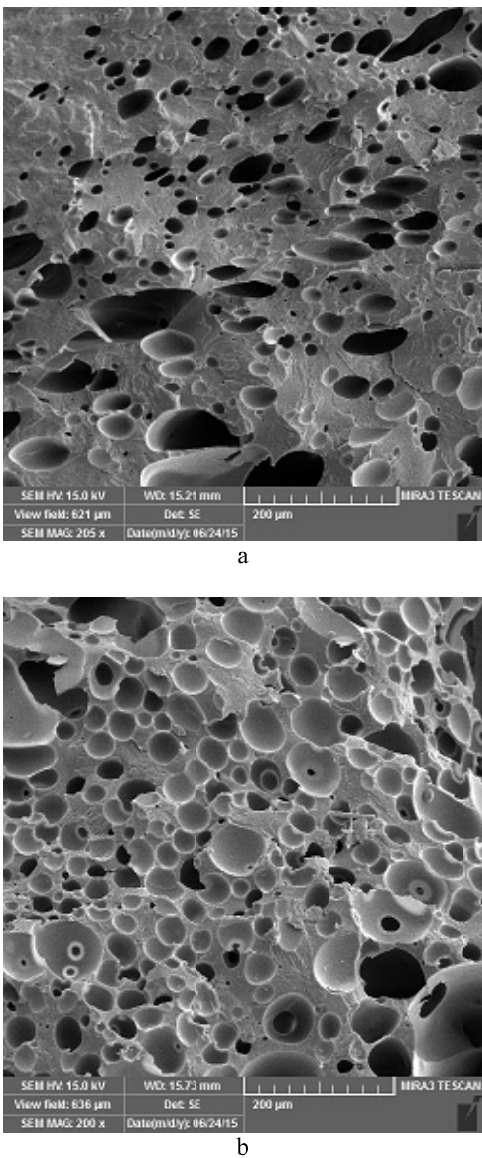
Fig. 2. SEM picture of nanocomposite foam samples, a) PA-6 containing 1 wt% MWCNT and b) PA-6 containing 1.5 wt% MWCNT
