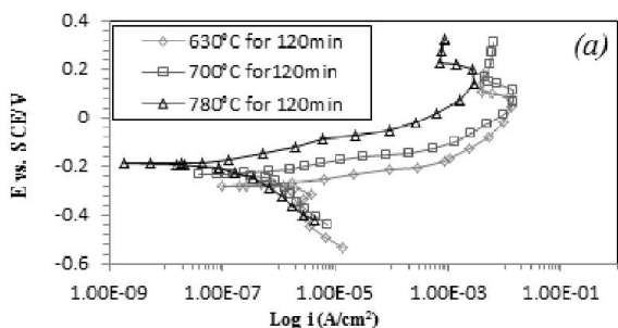
Fig. 4. Polarization curves of the alloys in 3.5% NaCl solution after different annealing temperatures and times: (a) ADB, (b) ALB.
