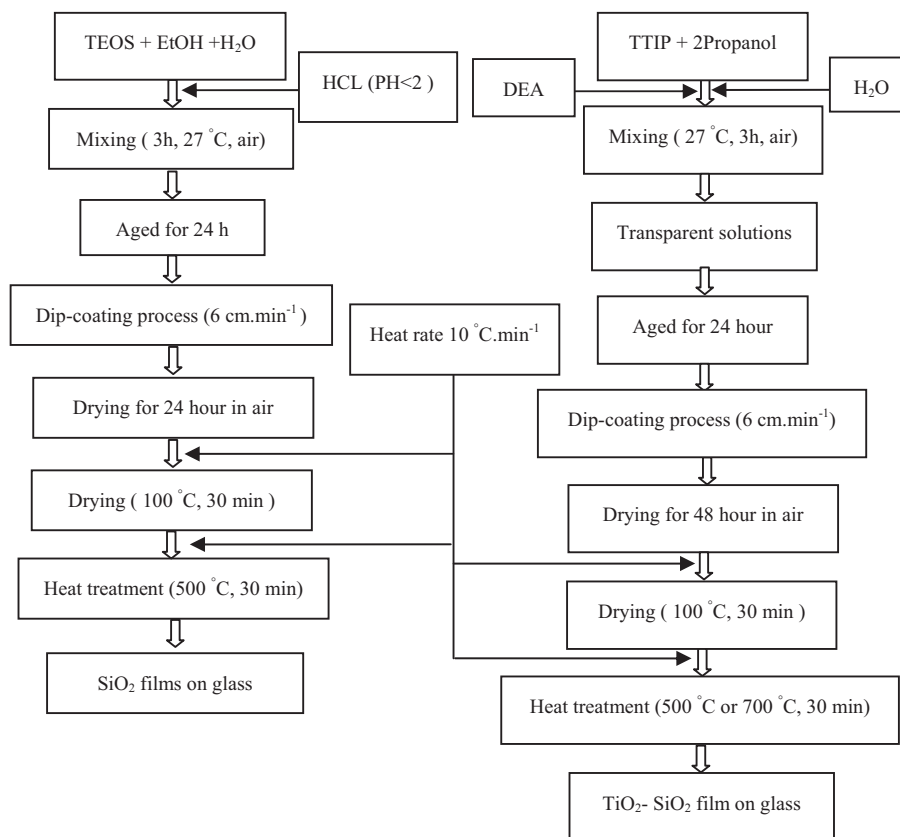
Fig. 1. Experimental procedure used in this research (left: preparation process of SiO 2 films, right: the preparation process of TiO 2 -SiO 2 films).
